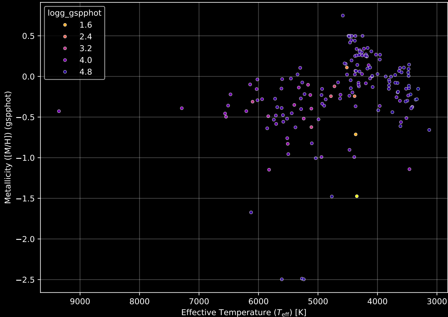
APOGEE DR17 Field: [SA57-N] Stellar Population Parameters (n= 169)
