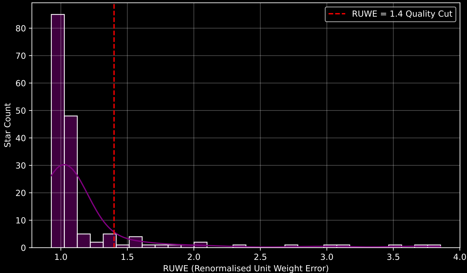
GAPOGEE DR17 Field [SA57-N] RUWE Distribution (n= 163)
