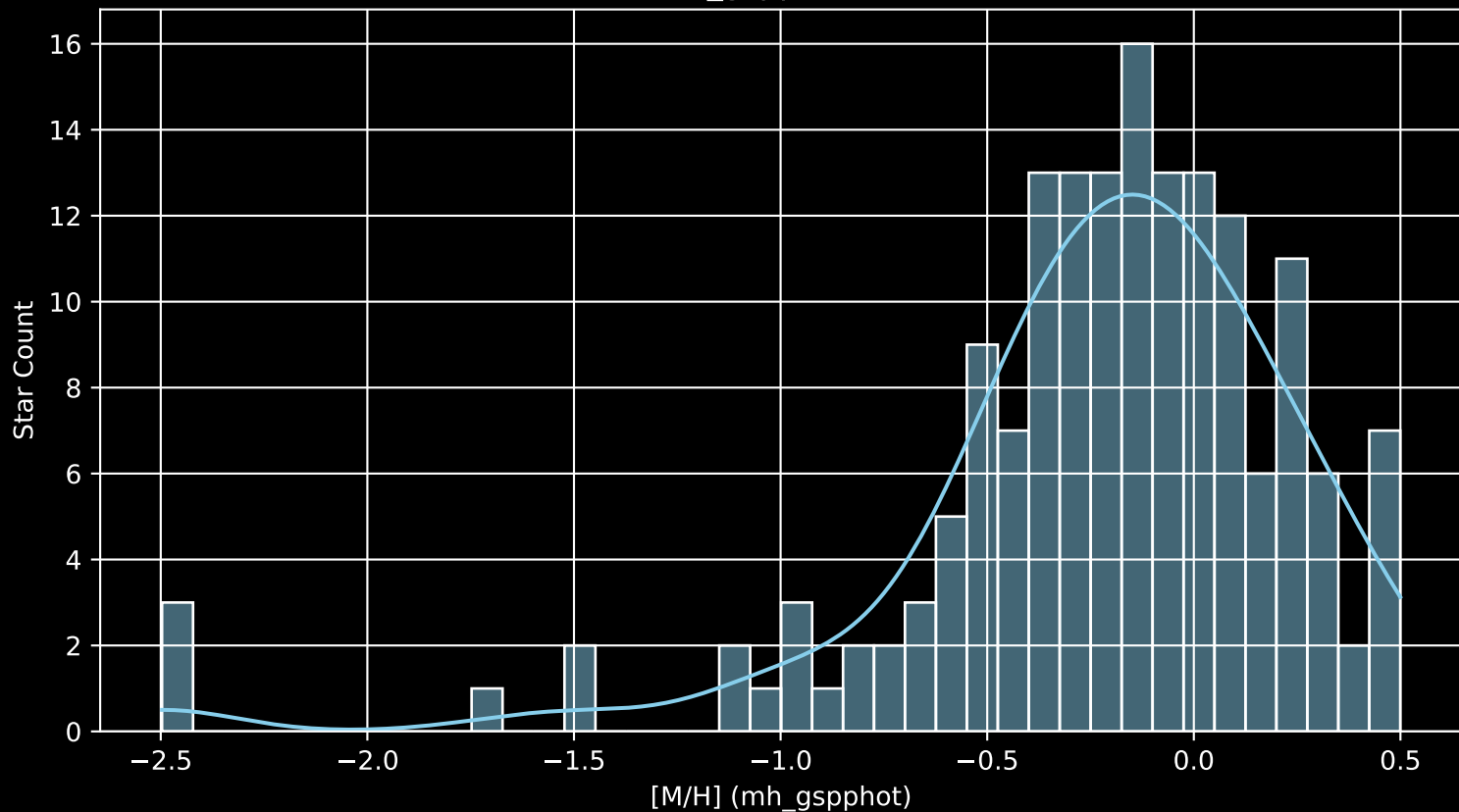
APOGEE DR17 Field: [SA57-N [M/H] (mh_gspphot) (n= 166)
