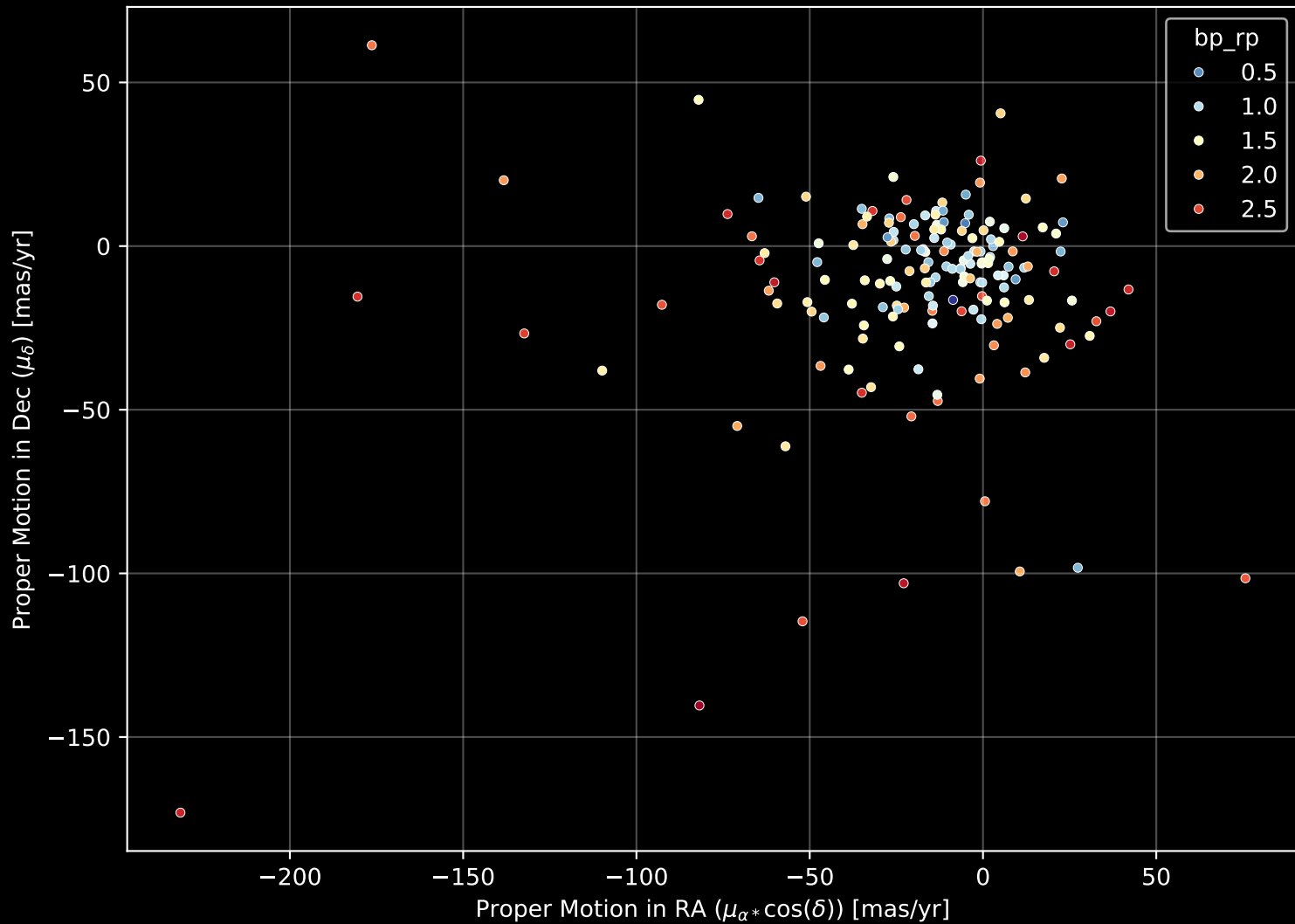
APOGEE DR17 Field: [SA57-N] Proper Motion Diagram (n= 169)
