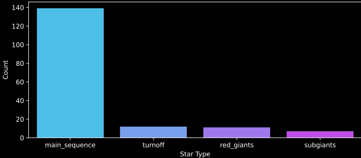
APOGEE DR17 Field: [SA57-N] Count plot of Star Type
