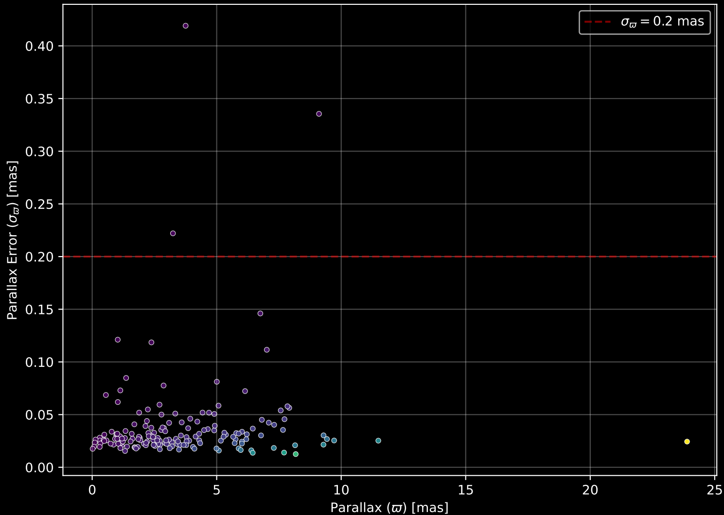
APOGEE DR17 Field: [SA57-N] Parallax Quality (n= 169)
