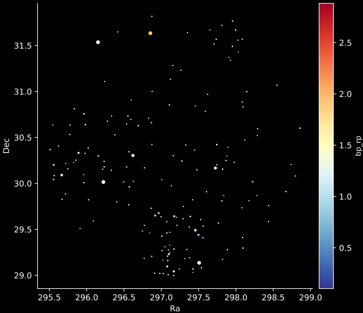
APOGEE DR17 Field: [SA57-N] Stars: 169
